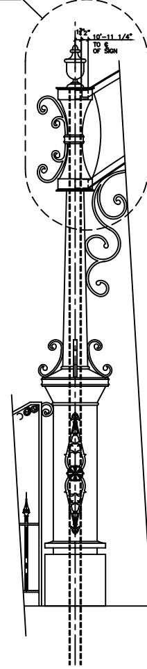
1 ENLARGED ELEVATION OF COLUMN D-2 SCALE: 1" = 1'-0"
